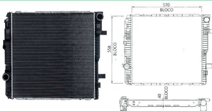
ATEGO 1315/1418/1518/1718 - S/L
