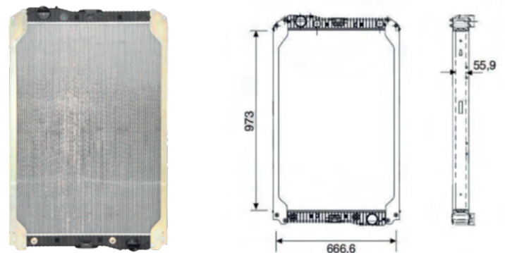
AXOR 2540/2640/2035/2040/2644 - C/L
