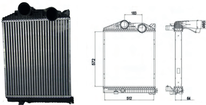
ATEGO 1315/1418/1518/1718/1719
